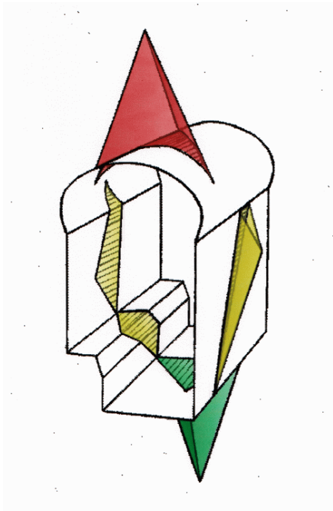
Figure 4: Perspective view of R o Grande power cavern showing potentially unstable wedges in the roof, sidewalls, bench and floor.
